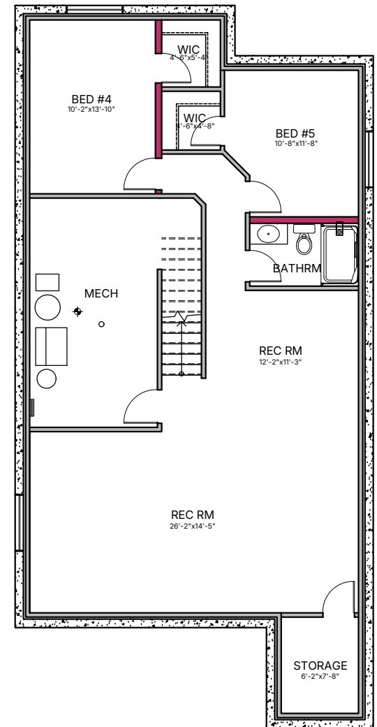
OPTIONAL FINISHED BASEMENT - 1,435 sq.ft.
